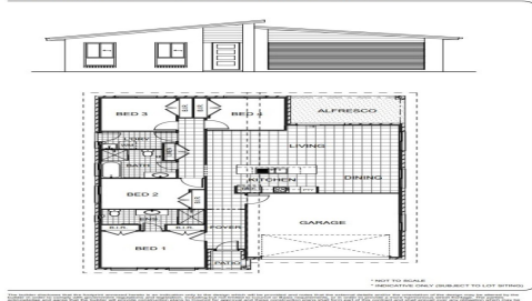
VERANO GEN V - F4 QM LOT 15 AREAS: Living - 146.3 m 2 | Garage - 37.0 m 2 | Patio - 2.4 m 2 | TOTAL 185.7 m 2
